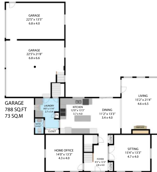
MAIN LEVEL 1,382 SQ.FT 128 SQ.M
